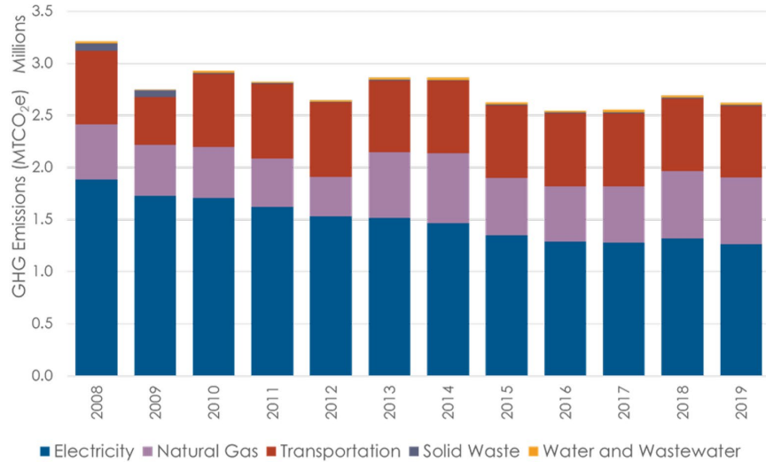
Figure 4. 2008-2019 Community GHG emissions
